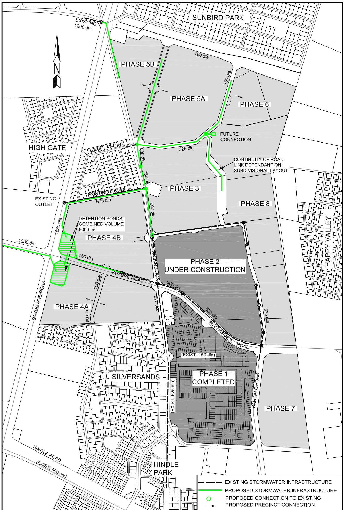
SILVERSANDS - BARDALE VILLAGE PROPOSED STORMWATER LAYOUT
